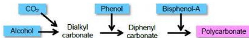
Figure 6 Carbonation of alcohol route
