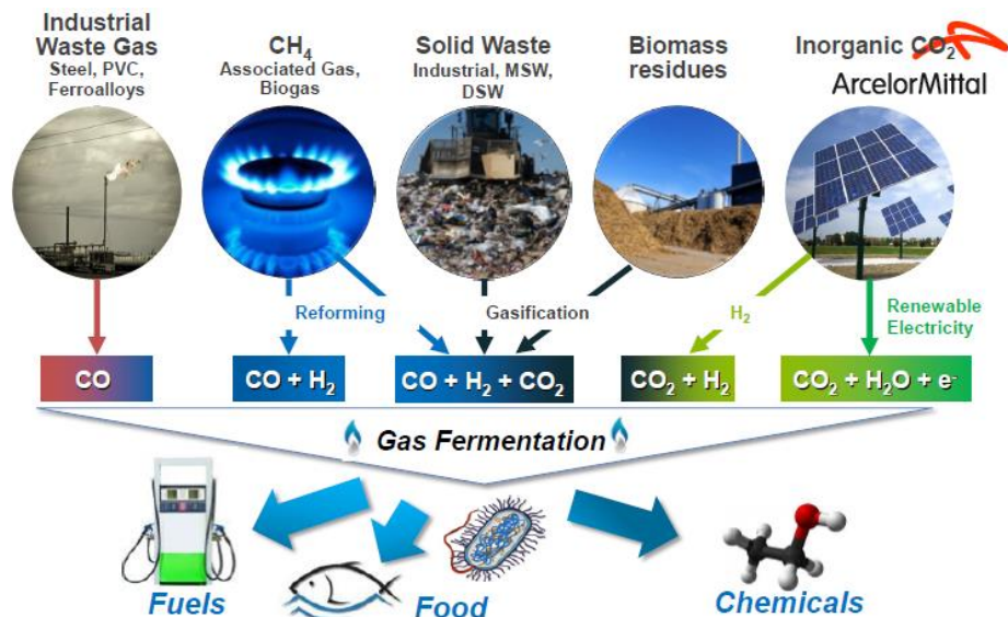
Figure 14 H 2 and CO/CO 2 to ethanol process routes
