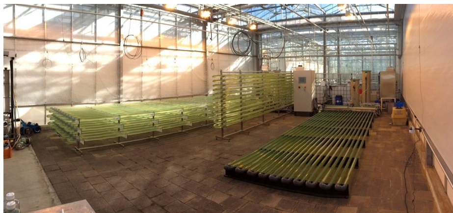
Figure 15 Closed tubular pilot reactors
