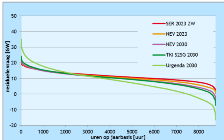
Figure 4 Demand and supply on the power grid
