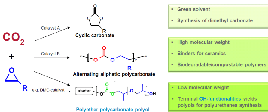
Figure 5 Carbonation of epoxides routes
